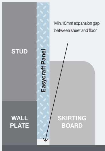
Installation of Mouldings, Cornices, Skirtings & Architraves Figure 7
