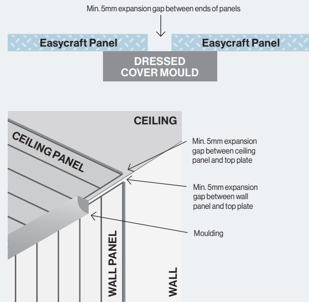
Installing Panels End to End Figure 8
