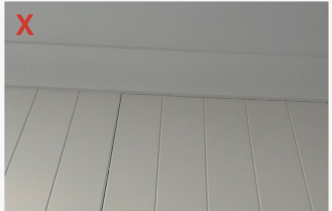
Tongue and groove joint showing due to no flexible paintable sealant being used
